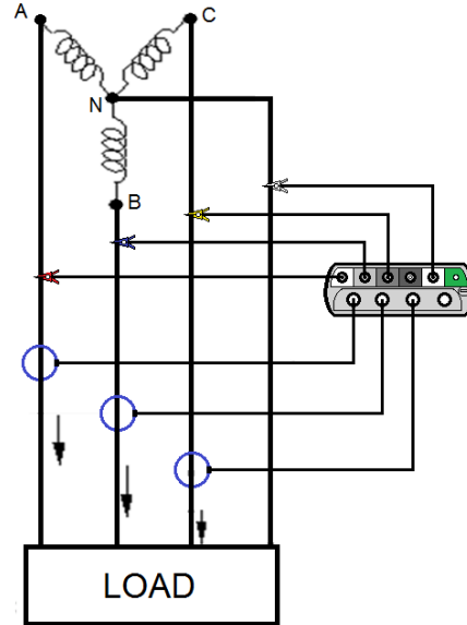
4 - Wire Wye Connection 3 - Wattmeter Method
