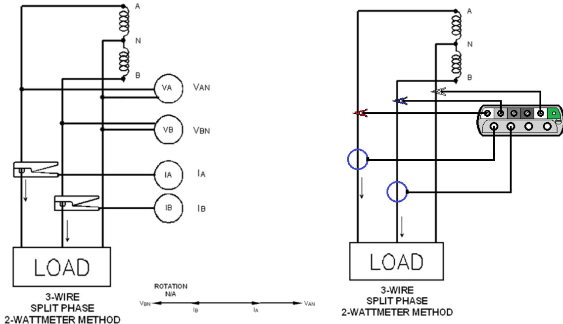
2 Wattmeter – (2 Voltage and 2 Current)
